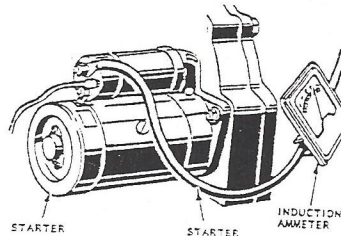
USING THE INDUCTION AMMETER TO TEST STARTER CURRENT
