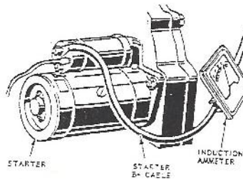
USING THE INDUCTION AMMETER TO TEST STARTER CURRENT
