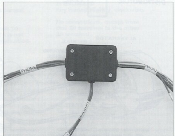
UHLtronics Triad module is inserted into the Saab wiring harness.
