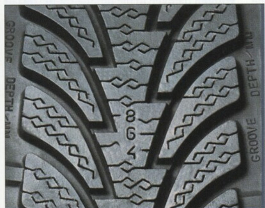
Close up of the WR tread, showing the Driving Safety Indicator (DSI) numbers molded into the tread and the geometry of the "Haka Siping".
