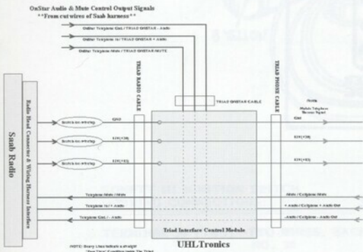
Block diagram shows how Triad interfaces with the Saab wiring.
