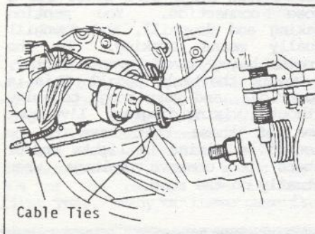
Figure 2. Overpressure switch relocated inside plastic housing.
