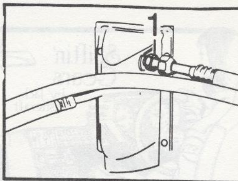
Evaporator as from 1984 model cars Copper = Borletti Aluminium = Sanden
